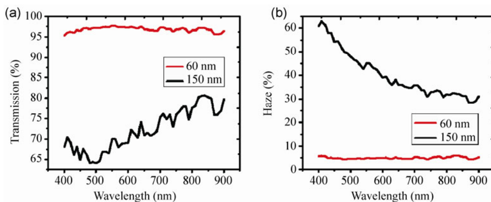
Figure 2 Simulation of (a) transmission and (b) haze factor of Ag NWs with different diameters (60 nm and 150 nm).
