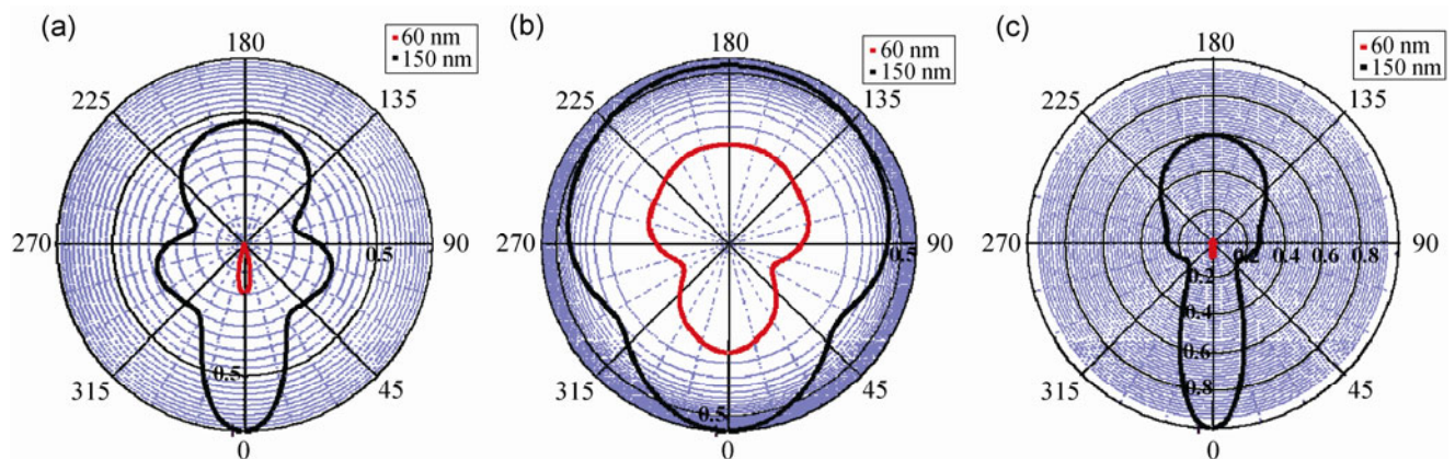
Figure 3 Simulation of the normalized scattered field intensity versus scattering angle from the axis normal to the silver nanowire with diffuse scattering represented by acute angles ( 0^{\circ} – 90^{\circ} and 270^{\circ} – 360^{\circ} ) and backscattering represented by obtuse angles ( 90^{\circ} – 270^{\circ} ) for (a) TE polarization and (b) TM polarization and (c) average of TE and TM for 60 nm and 150 nm diameter silver nanowires. (a) and (b) are in log scale and (c) is in linear scale for clarity.
