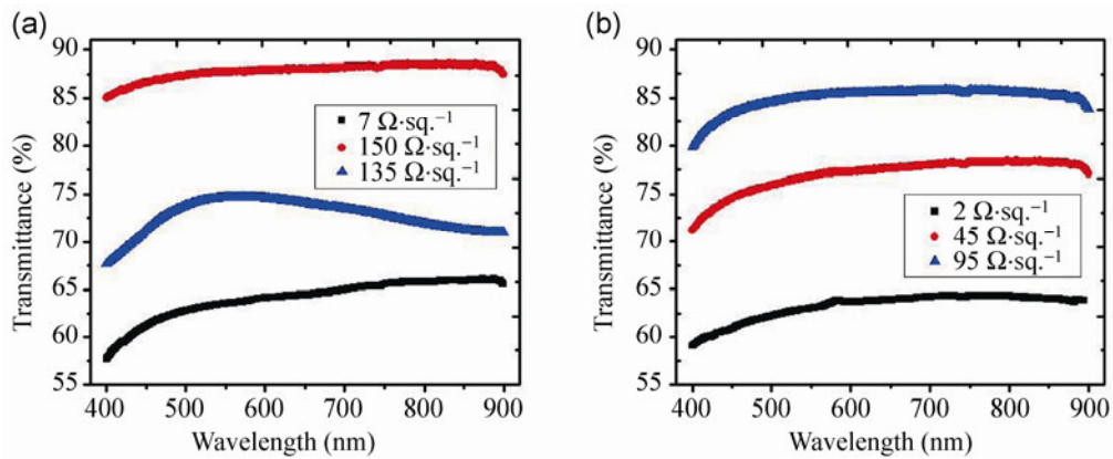
Figure 5 (a) The transmittance spectrum for the various films formed from vacuum filtration of Ag NW dispersions with large diameters (~150 nm). (b) The transmittance spectrum for the various films formed from vacuum filtration of Ag NW dispersions with small diameters (~60 nm).
