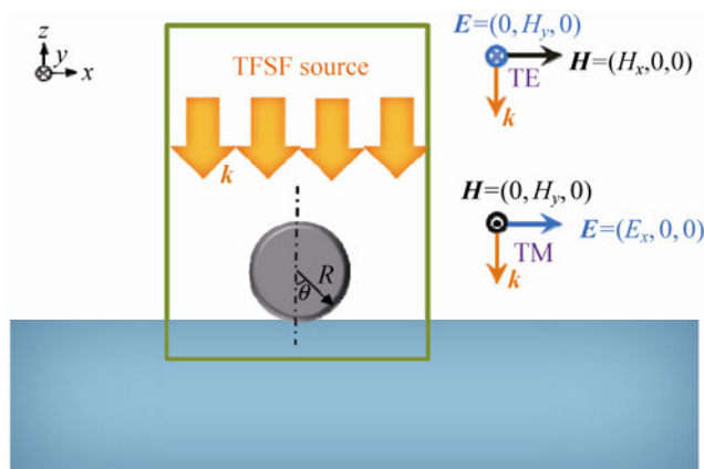
Figure 1 Schematic of the 2D simulation setup used to calculate the light scattering behavior at normal incidence from a single silver nanowire with a radius of R . The center of the nanowire is the origin of the axes. The green box represents a total field scattered field (TFSF) source with a length of 500 nm in the x -direction. The length is chosen according to the average spacing between Ag NWs as calculated from SEM images.
