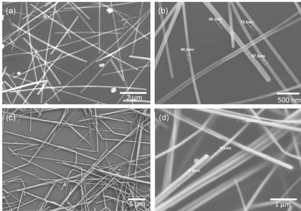
Figure 4 SEM images of Ag NWs: (a) percolation network of the film with small diameters; (b) display of small Ag NW diameters with little deviation, the diameters are as small as ~60 nm; (c) percolation network of film with large diameters; (d) display of large Ag NW diameters with little deviation, with an average of ~150 nm.
